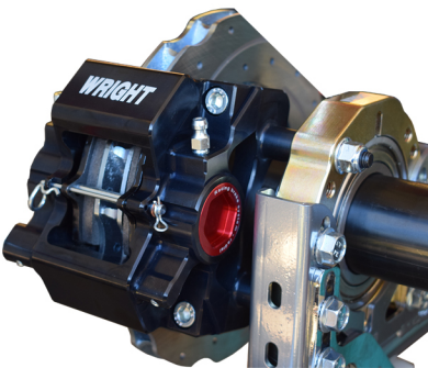
Mono Block Hydraulic Brake Caliper
