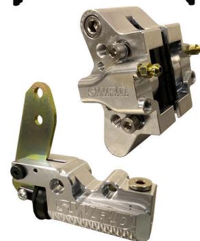
Phoenix Super Light Hydraulic Brake System
