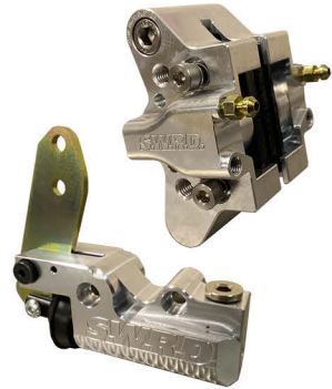
Phoenix Super Light Hydraulic Brake System
